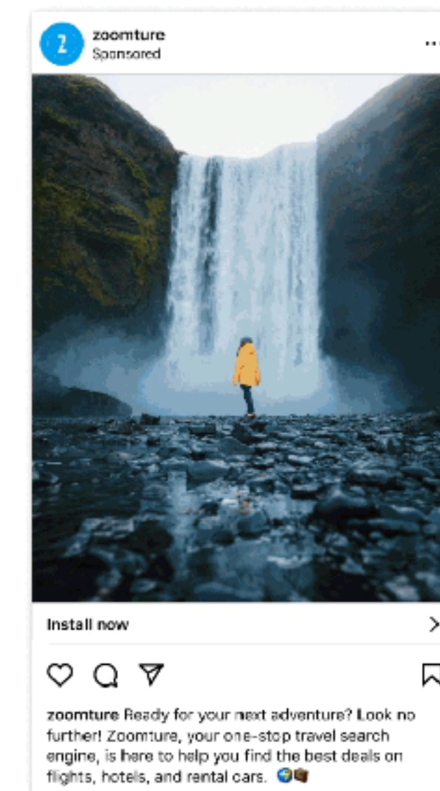
Text variations
