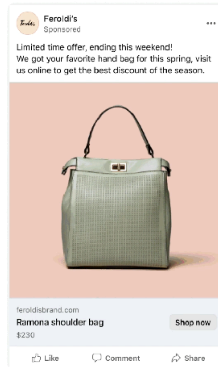
Background generation
